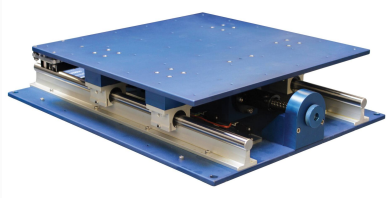
Shake Table, Single-Axis Bench- Scale PLMT-ST1
