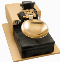
Liquid Limit Device Casagrande. Motorized
